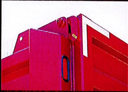
Heavy duty, greaseable steel removable tailgate hinge pin.
